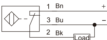
WD9 DC 3-wire PNP NC
