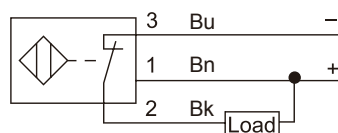
WD10 DC 3-wire NPN NC
