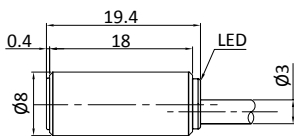
Fig. 1 Inductive sensor with cable (flush)
